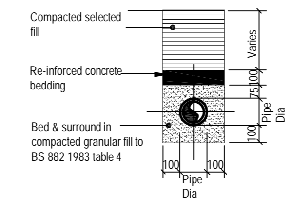
TYPICAL PIPE TRENCH FOR FOUL & SURFACE WATER DRAINS WHEN LAID UNDER ROADS WITH LESS THAN 900mm COVER
