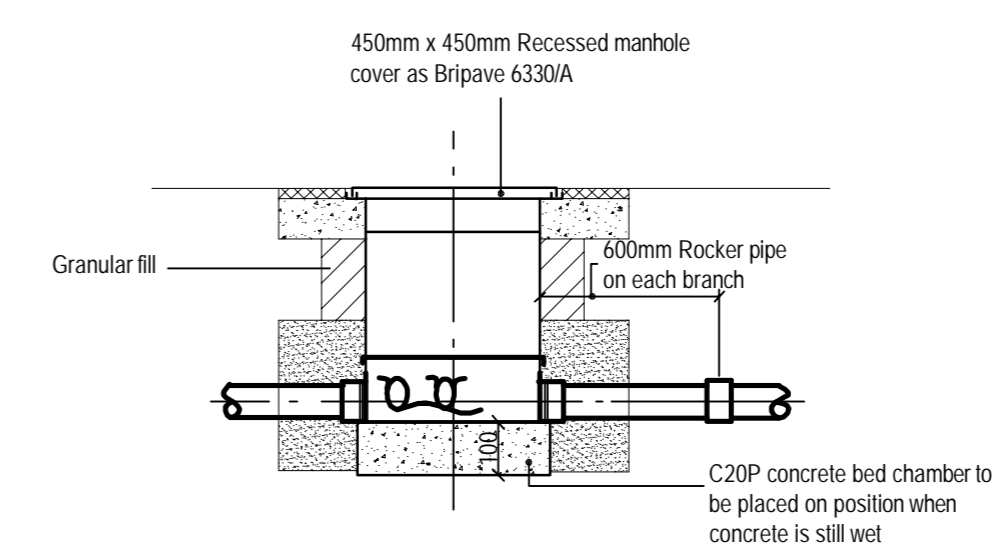
SECTION DETAIL OF MANHOLE
