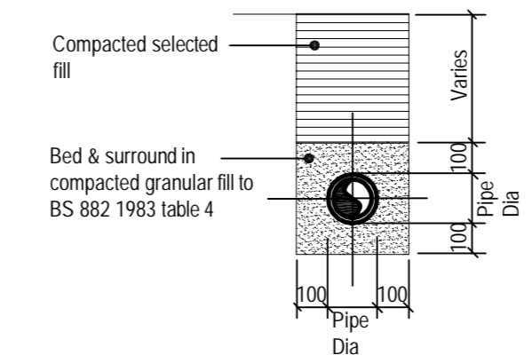
TYPICAL PIPE TRENCH FOR FOUL & SURFACE WATER DRAINS
