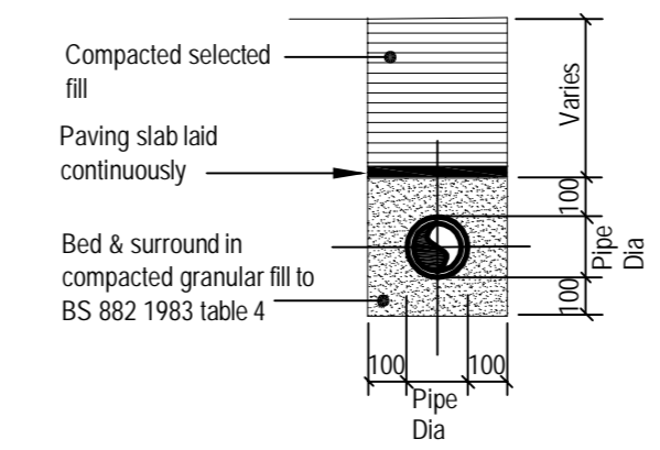
TYPICAL PIPE TRENCH FOR FOUL & SURFACE WATER DRAINS WHEN LAID WITH LESS THAN 600mm COVER
