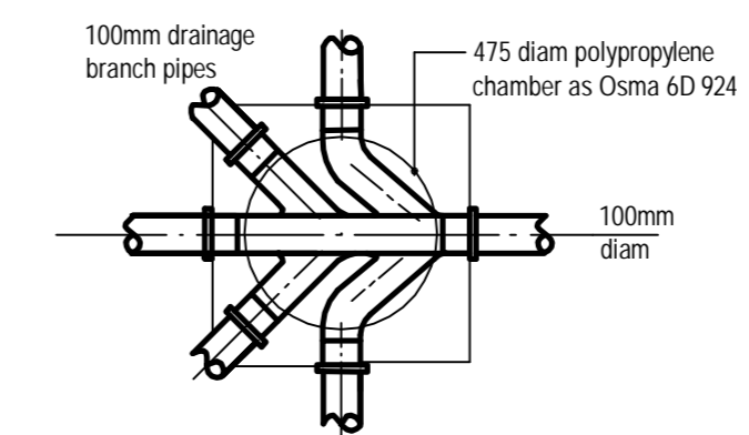
PLAN DETAIL OF MANHOLE
