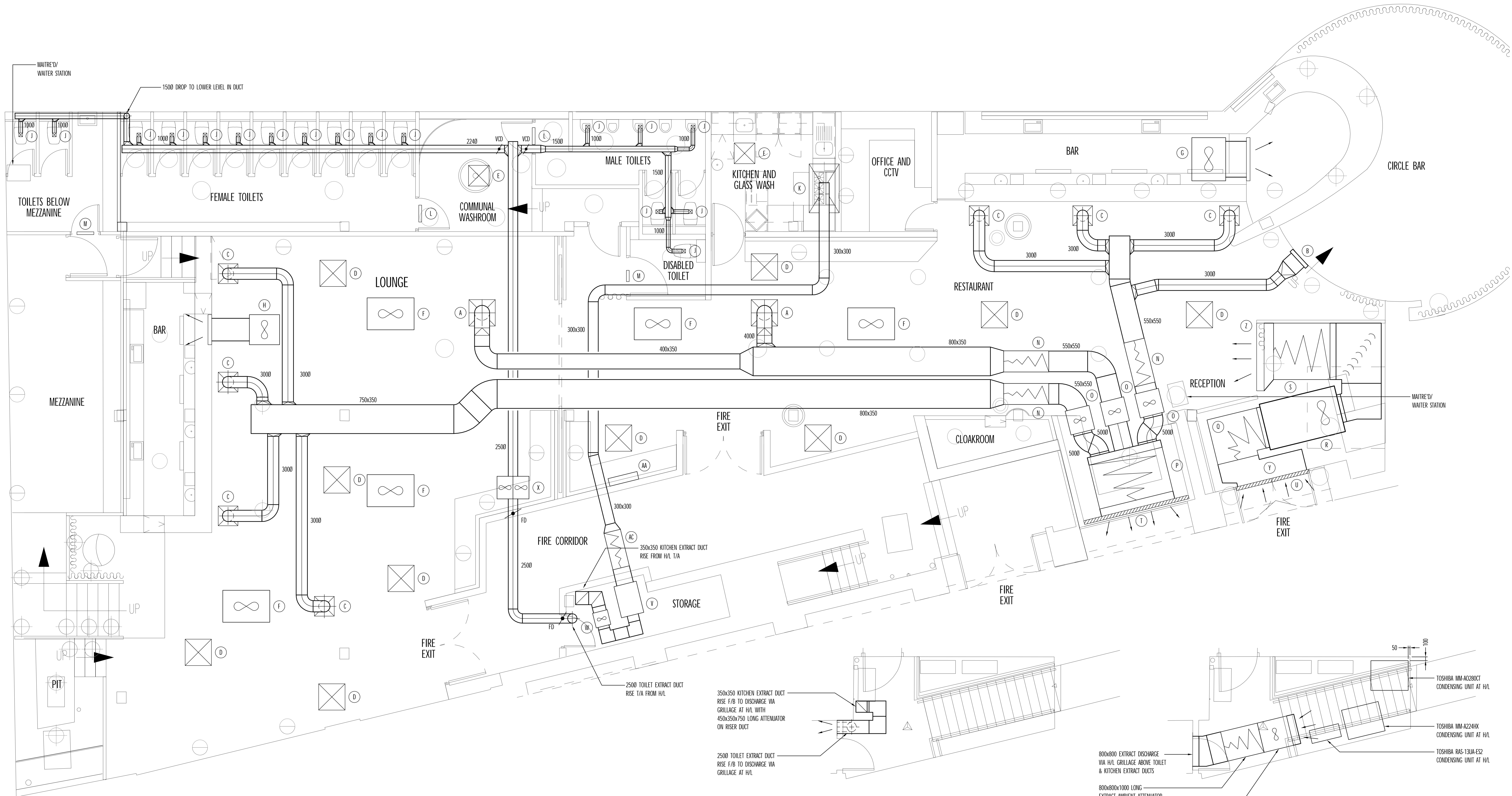
FIRST FLOOR PART PLAN KITCHEN & TOILET EXTRACT DUCTWORK
