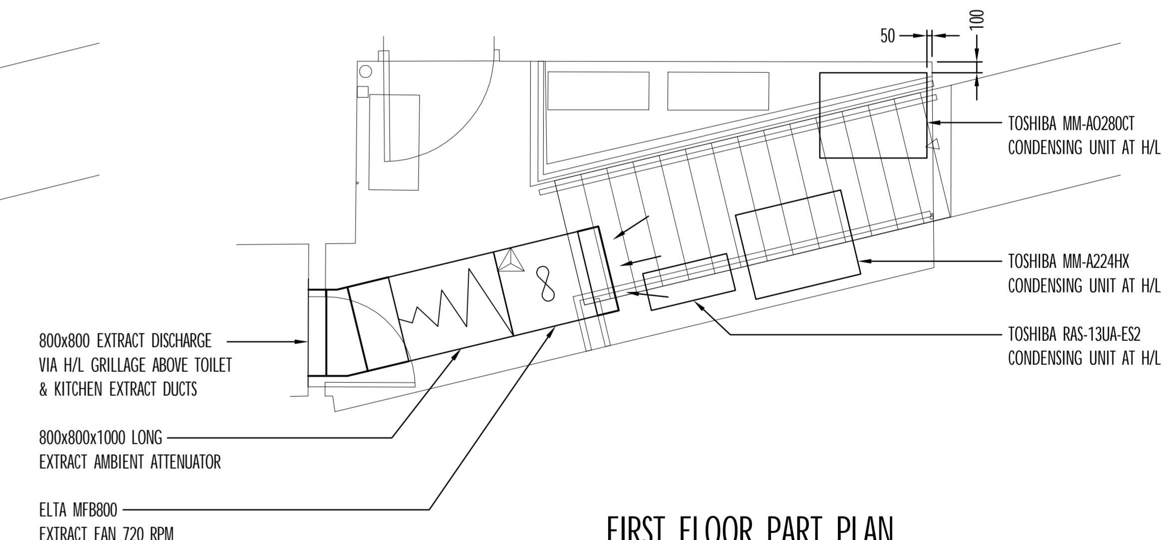
FIRST FLOOR PART PLAN CONDENSING UNITS
